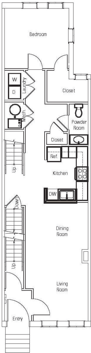
First Floor
