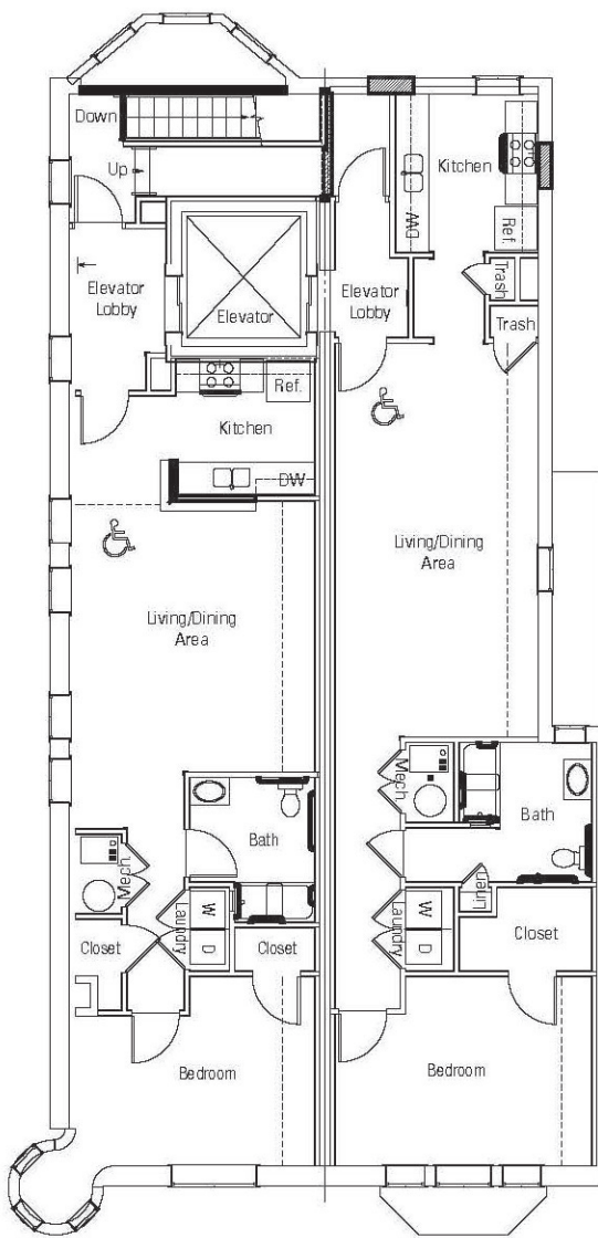
Third Floor
